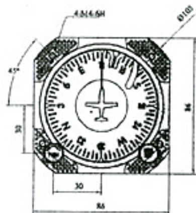
Panel Cut-out Sketch (For Rear Mounting)
