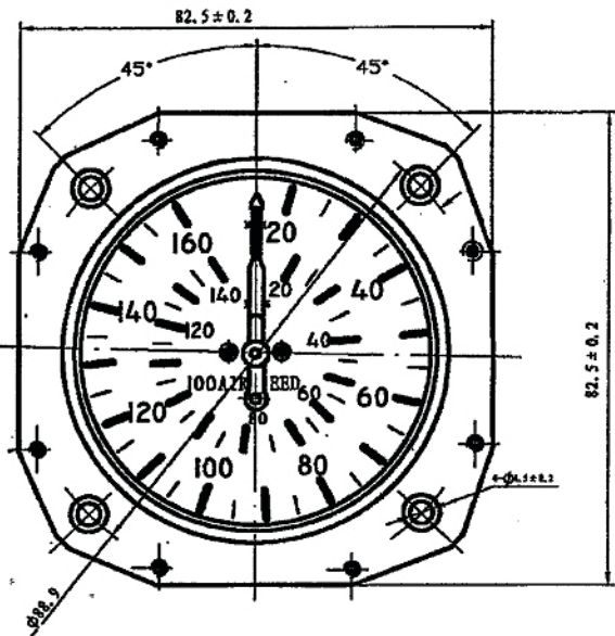
ASI164MN-3 3 1/8" Type Dual range Airspeed Indicator 20-160 mph/ 20-140 knots
