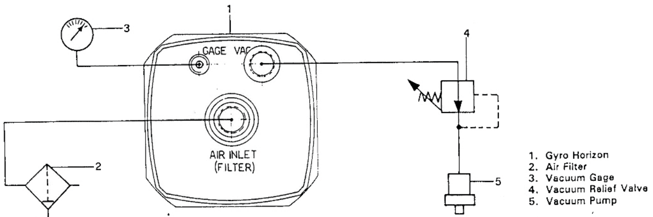
Figure 1.3-2. Installation Scheme - Typical
