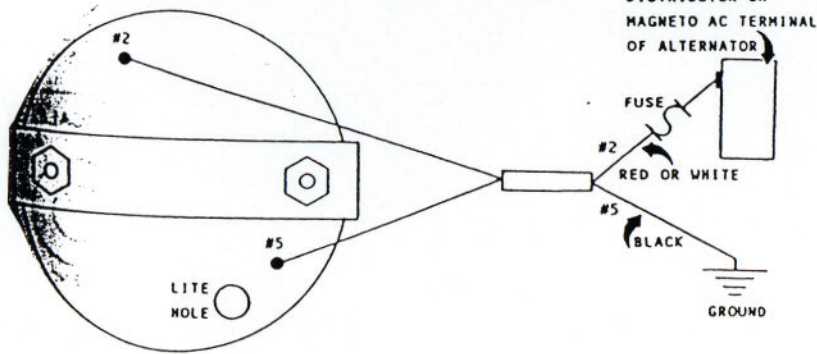
Tach Hook-up:
