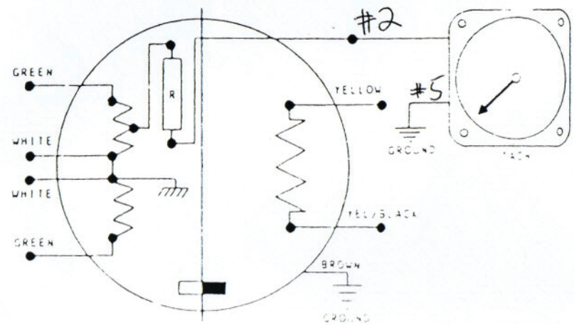
Wiring Diagram for Tachometer:
