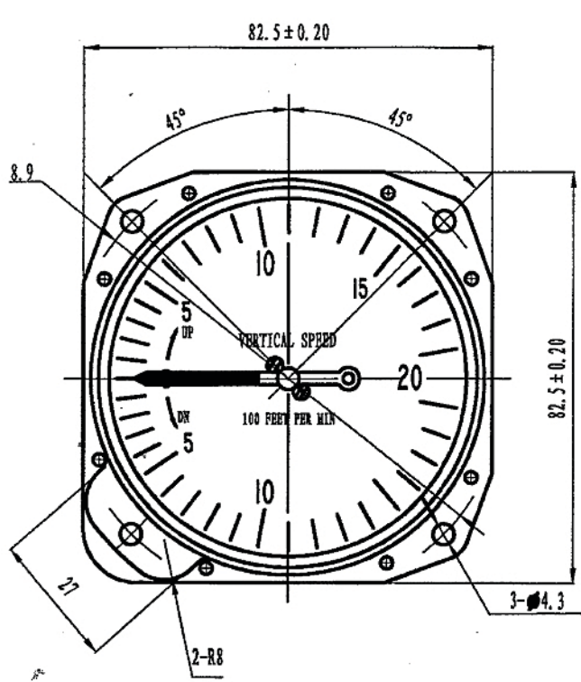
VSI2FM-3 3 1/8" type Vertical Speed Indicator 0-2000 ft.
